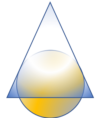
Conic
