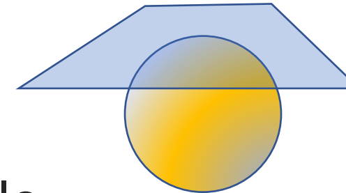
Azimuthal
